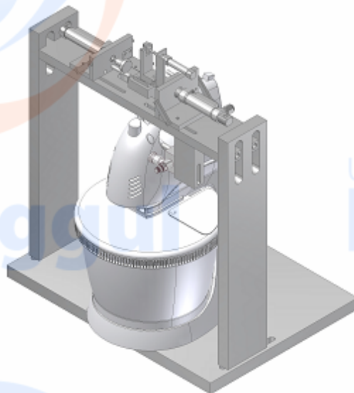
Mixer Switch Life Test
