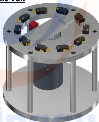
Microswitch Life Test
