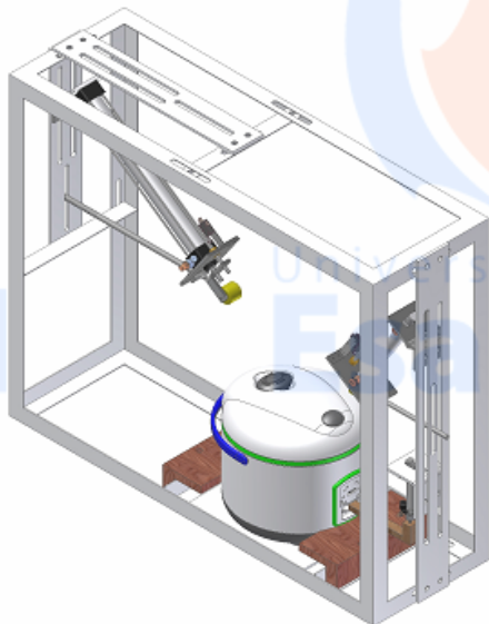
Switch Life Test
